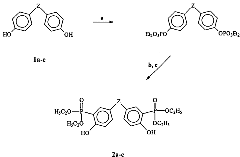
SCHEME 1 Reagents: a) \text{HP(O)(OC}_2\text{H}_5)_2/\text{CCl}_4 , \text{N(C}_2\text{H}_5)_3 , 0^\circ\text{C} ; b) \text{LDA/THF} , -78^\circ\text{C} ; c) saturated \text{NH}_4\text{Cl/H}_2\text{O}
